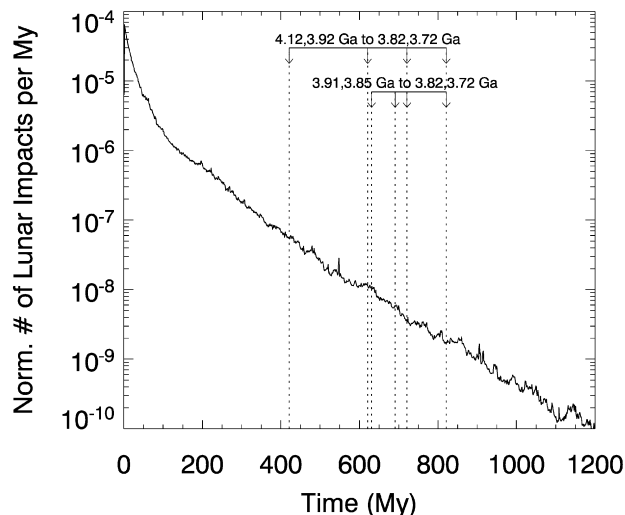
Fig. 5. The number of lunar impacts produced per My by the PPP, where the size of the PPP has been normalized to a single object. The t = 0 My time was assumed to be the Moon-forming event. The PPP impact rate drops sharply over the first 100 My and then transitions to a more steady decline between 100 to 1200 My. The largest lunar basins formed in Nectarian and early-Imbrium time periods are, in order of decreasing size, Imbrium, Orientale, Serenitatis, and Nectaris. The plausible formation intervals for basin sets A and B are given in Table 1. The interval with a maximum at 4.12 Ga and a minimum at 3.72 Ga corresponds to basin set A. The interval with maximum at 3.91 Ga and minimum at 3.72 Ga corresponds to basin set B. No basins formed after these times.
