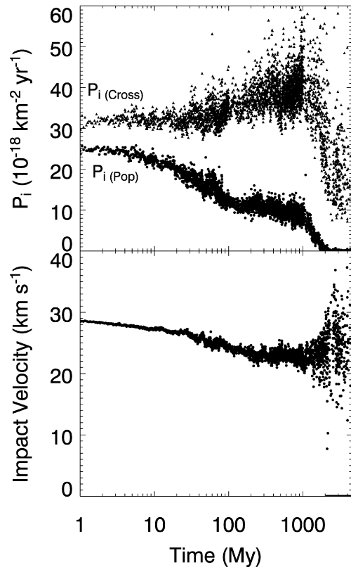
Fig. 4. The mean intrinsic collision probabilities (top) and impact velocities (bottom) between the Moon and test bodies in the PPP. The mean intrinsic collision probability of test bodies on Moon-crossing orbits is labeled as P_i(\text{Cross}) , while that of the entire population is P_i(\text{Pop}) . The difference between the two values over time shows that the longest-lived test bodies evolve away from Moon-crossing orbits. Note that P_i(\text{Cross}) and the mean impact velocity of test bodies on Moon-crossing orbits only changes by relatively small amounts throughout the simulation.
