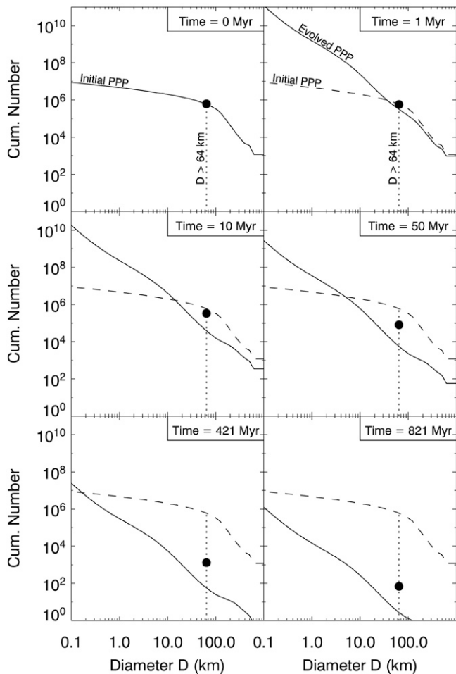
Fig. 9. The collisional evolution and dynamical depletion of the post-planet formation population (PPP) in which the initial mass is 0.6M_{\oplus} (see Section 4.3). The t = 0 My timestep shows the initial shape of the PPP size distribution, which was generated using results from Bottke et al. (2005a, 2005b). The dashed vertical line corresponds to D > 64 km projectiles, the size needed to make the four largest Nectarian and early-Imbrium basins. The black dot shows what the depletion of D > 64 km projectiles would be when collisional evolution is excluded. The bump observed in most frames near D \sim 2 –4 km is driven by asteroid disruption scaling law, which undergoes a transition at D \sim 0.2 km between the strength and gravity-scaling regimes. The intermediate timesteps show how quickly comminution can reduce the initial population in addition to the bodies lost from dynamical depletion. By the t = 421 and 821 My timesteps, collisional evolution has reduced the number of D > 64 km objects in the PPP by nearly a factor of 20 below the expected depletion produced by dynamics alone. Accordingly, only a few D > 64 km projectiles are left in the PPP to produce the large Nectarian and early-Imbrium basins in this interval.
