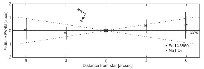
Fig. 4. Measured positions of the Na I and Fe I gas emission relative to the plane at position angle 30°.75. The bars correspond to derived scale heights, obtained by deconvolving the observed height profiles with a Gaussian of 0''.7 FWHM simulating the seeing. The inclined dash-dotted lines show the empirical opening angle of the gas disk, corresponding to H/r = 0.28 (see Sect. 5.1). The error in positioning of the slits is on the order of 0''.1.
