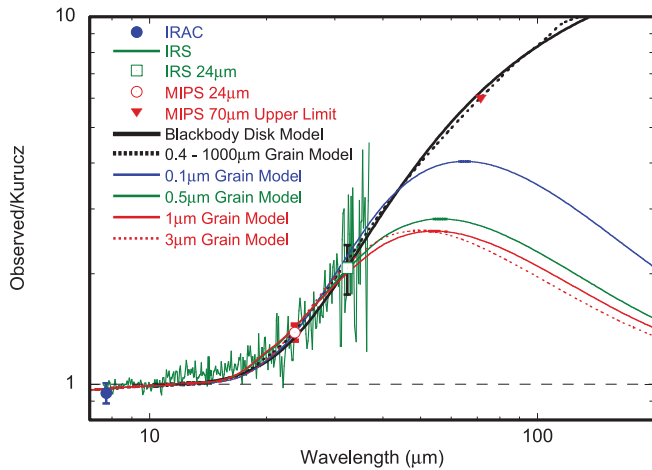
FIG. 6.—Spectrum of HD 12039 compared with spectra produced by the disk models from Table 2, all divided by the best-fit Kurucz model atmosphere. Several single-size-grain models are depicted as well as a model composed of grains with a power-law distribution of sizes from 0.4–1000 \mu\text{m} (Table 2; see text). The best-fit blackbody model is also shown for comparison. The single-size-grain dust models with particle sizes a \geq 7 \mu\text{m} from Table 2 are indistinguishable from the simple blackbody model and are not plotted independently in this figure.
