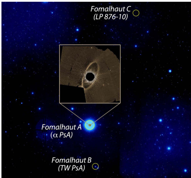
Figure 27. Fomalhaut system. North is up, east is left, and the sky-plane separation between Fomalhaut A and B is 2^{\circ} . The background image is a false-color, log-scale, gnomonic (tan) projection from the optical Digitized Sky Survey 1 (red plates), centered on \alpha = 344^{\circ}00 , \delta = -28^{\circ}00 (Credit: National Geographic Society, Caltech, STScI). The STIS Fomalhaut image is overlaid. (A color version of this figure is available in the online journal.)
