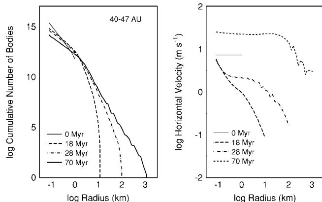
FIG. 6.—Evolution of a multiannulus coagulation model with \Sigma_i = 0.3 (a/35 \text{ AU})^{-3/2} , e_0 = 2 \times 10^{-3} , S_0 = 2 \times 10^6 \text{ ergs g}^{-1} , and velocity evolution: cumulative size distribution ( left ) and horizontal velocity ( right ) as a function of time. Collisional growth is quasi-linear until the largest bodies have r_{\text{max}} = 3\text{--}10 \text{ km} at 20 Myr. Collisional damping reduces the velocities of small bodies to \sim 1\text{--}5 \text{ m s}^{-1} on this timescale; dynamical friction reduces the velocities of larger bodies to \leq 10^{-1} \text{ m s}^{-1} . Runaway growth then produces objects with radii of 100 km in 10 Myr. Viscous stirring increases particle velocities as objects grow to sizes of 300–500 km, and runaway growth ends. An oligarchic growth phase leads to the production of 1000 km objects after \sim 70 \text{ Myr} ; the horizontal velocities are then \sim 40\text{--}50 \text{ m s}^{-1} for the smallest objects and \sim 2\text{--}3 \text{ m s}^{-1} for the largest objects.
