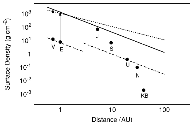
Fig. 2.—Surface density distribution in the solar system, assuming that the mass is spread uniformly over an annulus centered on the orbit of the planet. The arrows indicate the surface density for terrestrial planets if augmented to a solar abundance of hydrogen and helium. The solid and dot-dashed lines indicate \Sigma \propto A^{-3/2} (Weidenschilling 1977a; Hayashi 1981); the dashed line indicates \Sigma \propto A^{-1} (Cameron 1995).
