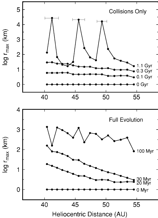
FIG. 7.—Mass of the largest body in each annulus of two multiannulus coagulation calculations. Top : Radius of the largest object at 0, 0.1, 0.3, and 1.1 Gyr for a model without velocity evolution. Bottom : Radius of the largest object at 0, 20, 30, and 100 Myr for a model with velocity evolution. Each annulus initially contains 0.1–1 km bodies with the surface density in solid material equivalent to a minimum-mass solar nebula. Objects grow faster in models with velocity evolution, but objects become larger in models without velocity evolution. The error bars in the top panel indicate the Hills radius R_H for each large body formed in the calculation without velocity evolution. Objects cannot accrete material beyond 2.4 R_H (see also Alexander & Agnor 1998; Kokubo & Ida 1998).
