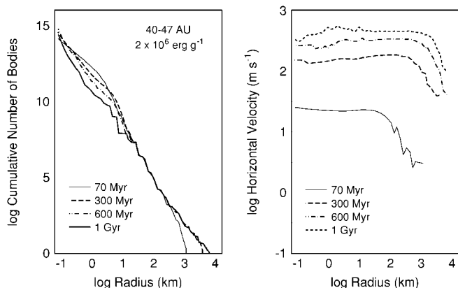
FIG. 9.—Late evolution of a multiannulus model with \Sigma_i = 0.3 (a/35 \text{ AU})^{-3/2} , e_0 = 2 \times 10^{-3} , S_0 = 2 \times 10^6 \text{ ergs g}^{-1} , and velocity evolution: cumulative size distribution ( left ) and horizontal velocity ( right ) as a function of time. After the first Pluto-sized object forms at \sim 70 Myr, growth is oligarchic. As objects grow from radii of \sim 1000 km to radii of \sim 6000 km, viscous stirring increases particle velocities to the shattering limit. Shattering reduces the population of 1–10 km objects on timescales of 500 Myr to 1 Gyr.
