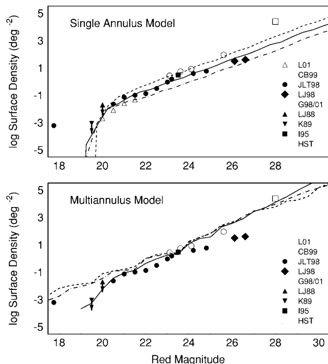
FIG. 11.—Comparison of model luminosity functions of KBOs with observations. Data are as indicated in the legend of each panel and are from Cochran et al. (1998; HST ), Irwin, Tremaine, & Zytlow (1995; I95), Kowal (1989; K89), Luu & Jewitt (1988; LJ88), Gladman et al. (1998, 2001; G98/01), Luu & Jewitt (1998; LJ98), Jewitt et al. (1998; JLT98), Chiang & Brown (1999; CB99), and Larsen et al. (2001; L01). Error bars for each datum (typically a factor of 2–3) and the upper limit from Levison & Duncan (1990) are not shown for clarity. The curves plot luminosity functions for ( top ) single-annulus models at 35 AU with e_0 = 10^{-3} and M_0 \approx 0.3 ( dot-dashed curve ), 1.0 ( solid curve ), and 3.0 ( dashed curve ) times the minimum-mass solar nebula and ( bottom ) multiannulus models at 40–55 AU for models with a mass in solids of a minimum-mass solar nebula with e_0 = 2 \times 10^{-3} and S_0 = 2 \times 10^6 ergs g^{-1} ( solid curve : 70 Myr; dashed curve : 1 Gyr) and S_0 = 10^3 ergs g^{-1} ( dot-dashed curve : 1 Gyr).
