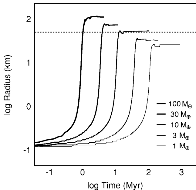
FIG. 5.—Evolution of r_5 , the radius where the cumulative number of objects is 10^5 , with time as a function of initial mass, M_0 , for single-annulus models with e_0 = 10^{-3} . The horizontal dashed line indicates the constraint on r_5 set by current observations. Adapted from Kenyon & Luu (1999a).
