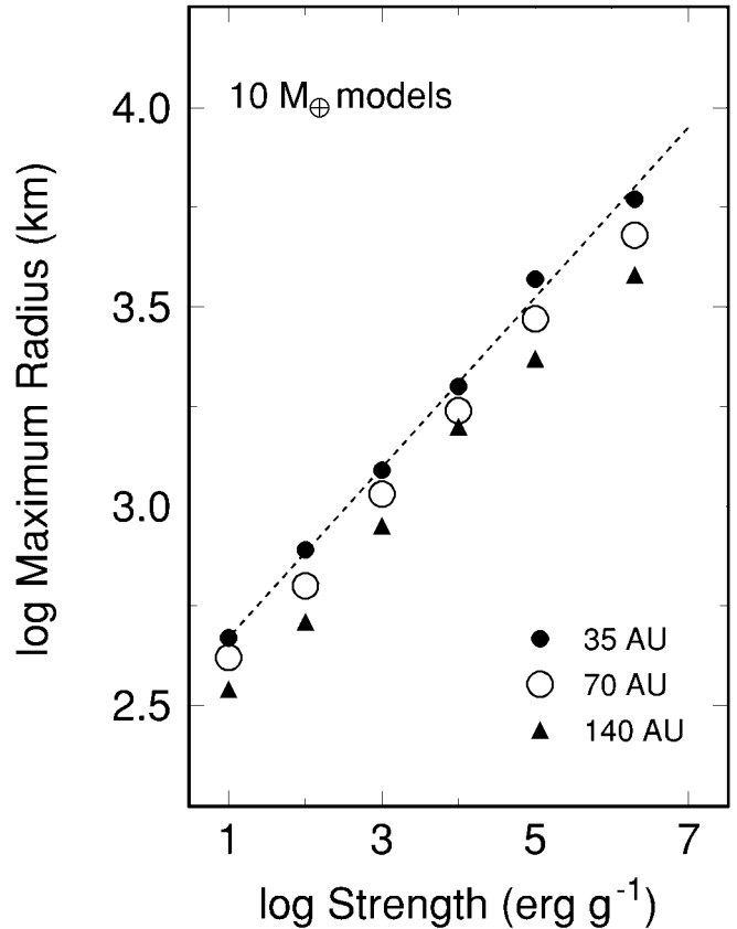
FIG. 4.—Maximum radius as a function of tensile strength and heliocentric distance for single-annulus models with M_0 = 10 M_{\oplus} and e_0 = 10^{-4} . At a given heliocentric distance, larger planets grow from stronger planetesimals. At a given tensile strength, smaller planets form at larger heliocentric distances. Adapted from Kenyon & Luu (1999a).
