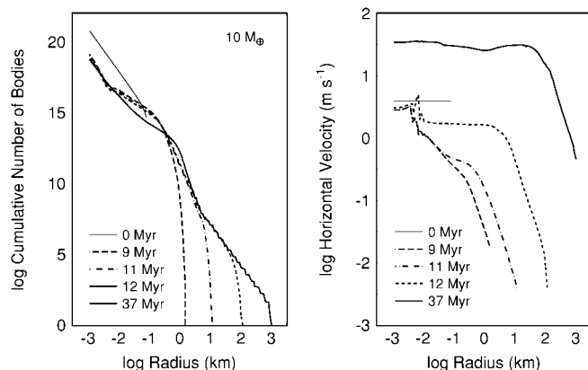
FIG. 3.—Evolution of a single-annulus coagulation model with M_0 = 10 M_\oplus , e_0 = 10^{-3} , and S_0 = 2 \times 10^6 \text{ ergs g}^{-1} : cumulative size distribution (left) and horizontal velocity (right) as a function of time. Collisional growth is quasi-linear until the largest bodies have r_{\text{max}} = 1\text{--}2 km at 9–10 Myr. Collisional damping reduces the velocities of all bodies to \sim 1\text{--}2 \text{ m s}^{-1} on this timescale; dynamical friction damps the velocities of larger bodies to \sim 10^{-2} \text{ m s}^{-1} . Runaway growth then produces objects with radii of 100 km in another 2–3 Myr. Viscous stirring heats up particle velocities as objects grow to sizes of 100–300 km. Runaway growth ends. A prolonged oligarchic growth phase leads to the production of 1000 km objects; the horizontal velocities are then \sim 30\text{--}40 \text{ m s}^{-1} for the smallest objects and \sim 1 \text{ m s}^{-1} for the largest objects. Adapted from Kenyon & Luu (1999a).
