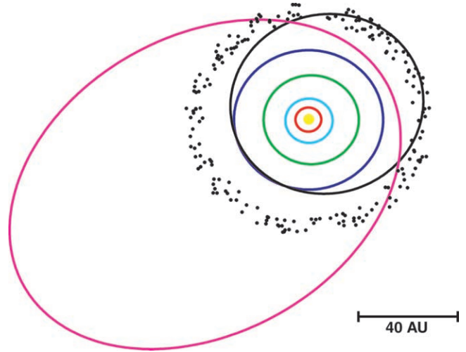
FIG. 1.—Top view of the solar system. The yellow filled circle is the Sun. Colored ellipses indicate the orbits of Jupiter ( red ), Saturn ( cyan ), Uranus ( green ), Neptune ( dark blue ), Pluto ( black ), and the scattered KBO 1996 TL 66 ( magenta ). The black dots represent 200 classical KBOs randomly distributed in a band between 42 and 50 AU. The bar at the lower right indicates a distance of 40 AU.
