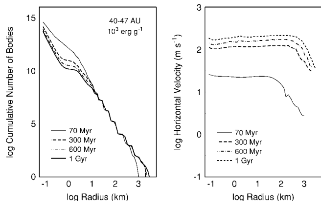
FIG. 10.—Late evolution of a multiannulus model with \Sigma_i = 0.3 (a/35 \text{ AU})^{-3/2} , e_0 = 2 \times 10^{-3} , S_0 = 10^3 \text{ ergs g}^{-1} , and velocity evolution: ( left ) cumulative size distribution and ( right ) horizontal velocity as a function of time. After the first Pluto-sized object forms at \sim 70 Myr, growth is oligarchic. As objects grow from radii of \sim 1000 km to radii of \sim 3000 km, viscous stirring increases particle velocities to the shattering limit. At times of 300 Myr to 1 Gyr, shattering reduces the population of small objects and produces a prominent dip in the size distribution at 0.3–3 km.
