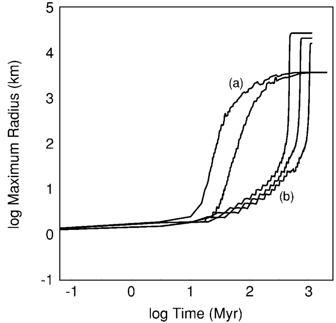
FIG. 8.—Evolution of the largest objects in several multiannulus calculations of planetesimal evolution at 40–55 AU. The two curves labeled “(a)” show the growth of the largest objects in a multiannulus calculation with velocity evolution and fragmentation (Fig. 6). The first curve plots the growth of the largest object in annulus 1; the second curve plots the growth of the largest object in annulus 15. The curves labeled “(b)” show the growth of the largest objects in a calculation with fragmentation but no velocity evolution (Fig. 7). The largest object in annulus 2 reaches runaway growth before the largest object in annulus 7, which achieves its maximum radius before the largest object in annulus 11 begins runaway growth.
