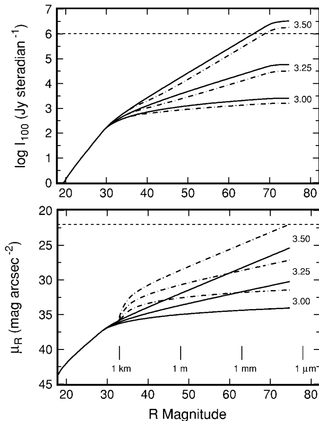
FIG. 12.—Far-IR and optical surface brightness as a function of R magnitude for a physical model of KBO grains. The model assumes a broken power-law size distribution, eq. (11), albedo \omega_g , and a surface density distribution for KBOs in a ring at 40–50 AU. Solid curves show results for a_1 = 3 , \omega = 0.04 , and a_2 as indicated at the right end of each curve. Dot-dashed curves repeat this model for small grains with larger \omega . Each model is consistent with observations of the optical counts at R \leq 26\text{--}27 . Adapted from Kenyon & Windhorst (2001).
