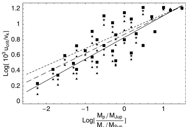
Fig. 7. Critical relative velocity of fragments u_{\text{crit}}/v_k to stay in the resonance, as a function of the planet-to-star mass ratio. Symbols: results of individual runs; lines: power law fits (33). Different maximum A of particles were adopted as a criterion of staying in the resonance: A = 30^\circ (triangles and solid line), A = 40^\circ (squares and dashed line), A = 50^\circ (stars and dotted line).
