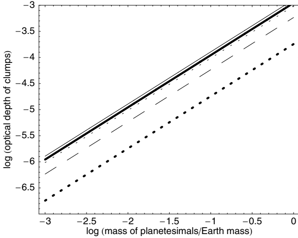
Fig. 8. Normal optical depth of the resonant clumps \tau in scenario II, as a function of the planetesimal population mass M . Thick lines are for u_0 = 5 \text{ m s}^{-1} and different \alpha : Dohnanyi’s \alpha = 0.833 (dashed) and a more realistic \alpha = 0.87 (solid). Thin lines are for \alpha = 0.87 and different u_0 and \gamma : u_0 = 1 \text{ m s}^{-1} and \gamma = 2 (solid), u_0 = 10 \text{ m s}^{-1} and \gamma = 2 (dashed), u_0 = 5 \text{ m s}^{-1} and \gamma = 1.5 (dotted). Cf. Fig. 4 for scenario I.
