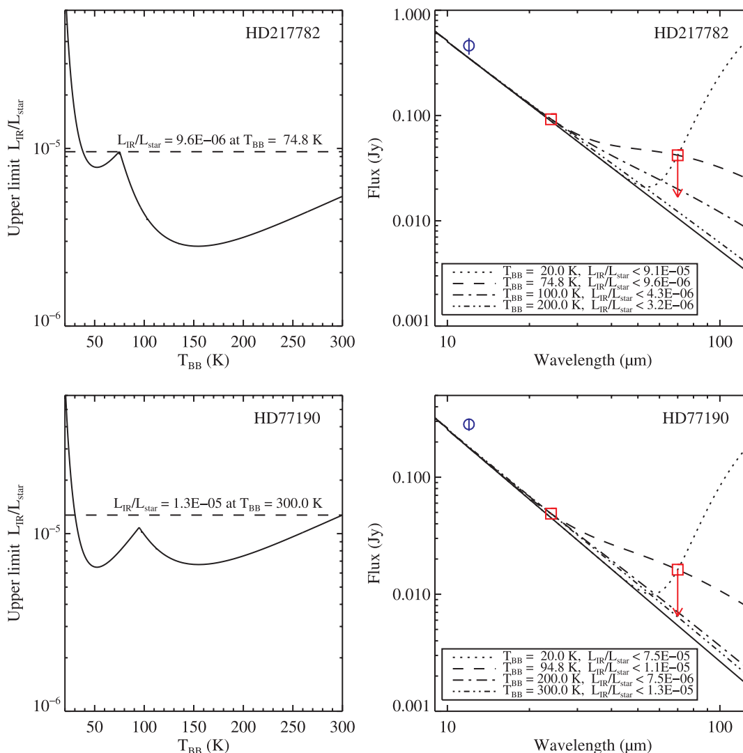
FIG. 3.— L_{\text{IR}}/L_{\text{star}} upper limits as a function of blackbody temperature. Left : L_{\text{IR}}/L_{\text{star}} upper limits for HD 217782 and HD 77190 plotted vs. T_{\text{BB}} . The largest L_{\text{IR}}/L_{\text{star}} upper limits for 50 \text{ K} < T_{\text{BB}} < 300 \text{ K} are indicated with horizontal dashed lines. Right : Portions of the SEDs of these two stars. The best-fitting upper limit SED models for four values of T_{\text{BB}} are overplotted with dotted, dashed, and dot-dashed lines. The color-corrected IRAS 12 \mu\text{m} flux is plotted with a blue circle. The MIPS 24 and 70 \mu\text{m} fluxes are plotted with red squares; 70 \mu\text{m} upper limits are indicated by arrows. See § 4.2 for a discussion of this figure.
