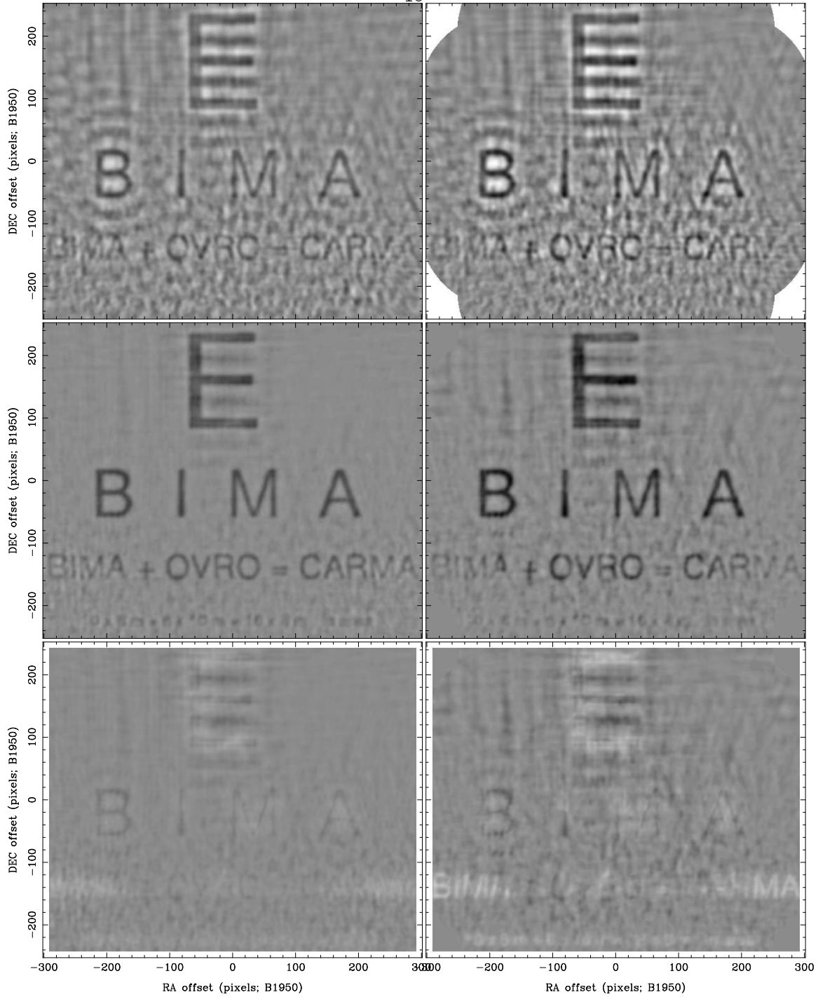
Fig. 8.— Effect of undersampling the pointing positions. The left column shows mosaic images with 19 pointings at 100 GHz sampled at the Nyquist interval with 6.1 m antennas. The right column shows the same images and sample interval using the primary beam of the 10.4 m antennas. The middle row shows the deconvolved images. The RMS residual (bottom row) is 50% worse with the undersampled pointing positions.
