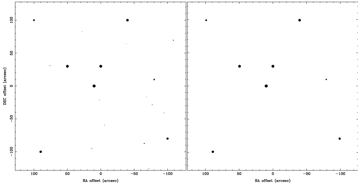
Fig. 2.— Eight point sources imaged with 2000 (left) and 4000 (right) uv samples. Logarithmic contours starting at 0.3%. With 2000 uv samples there are several spurious sources at the 0.3% level. With 4000 uv samples there are no spurious sources at the 0.3% level, although there is a 20% error in the measured flux density of the 10 mJy source.
