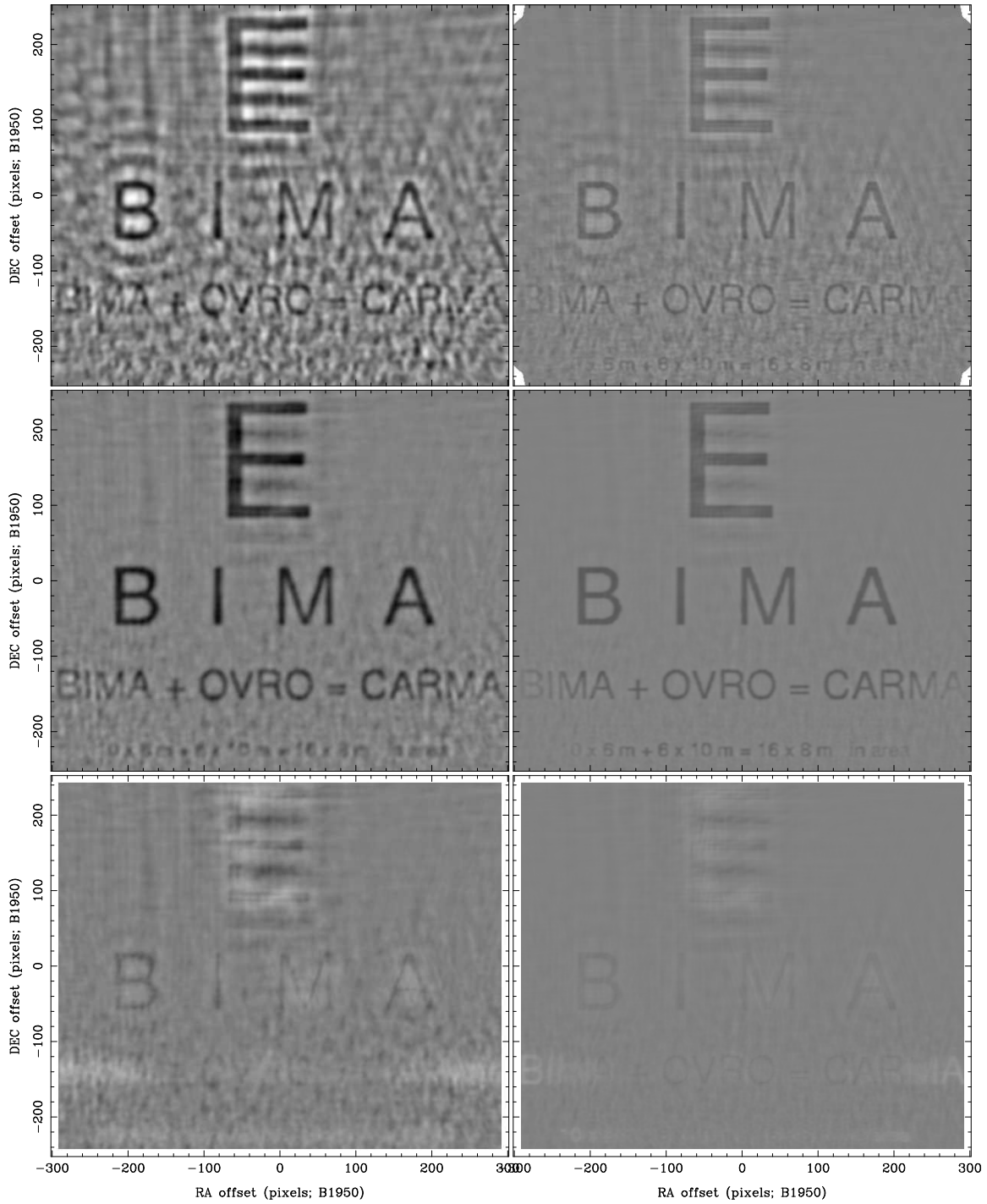
Fig. 7.— Eye chart imaged with current 10-antenna BIMA array (left) and 15-antenna CARMA array (right). Mosaic images imaged with 19 pointings at 100 GHz (top row). Deconvolved images (middle row). The RMS residual (bottom row) is 3\times better with the CARMA array.
