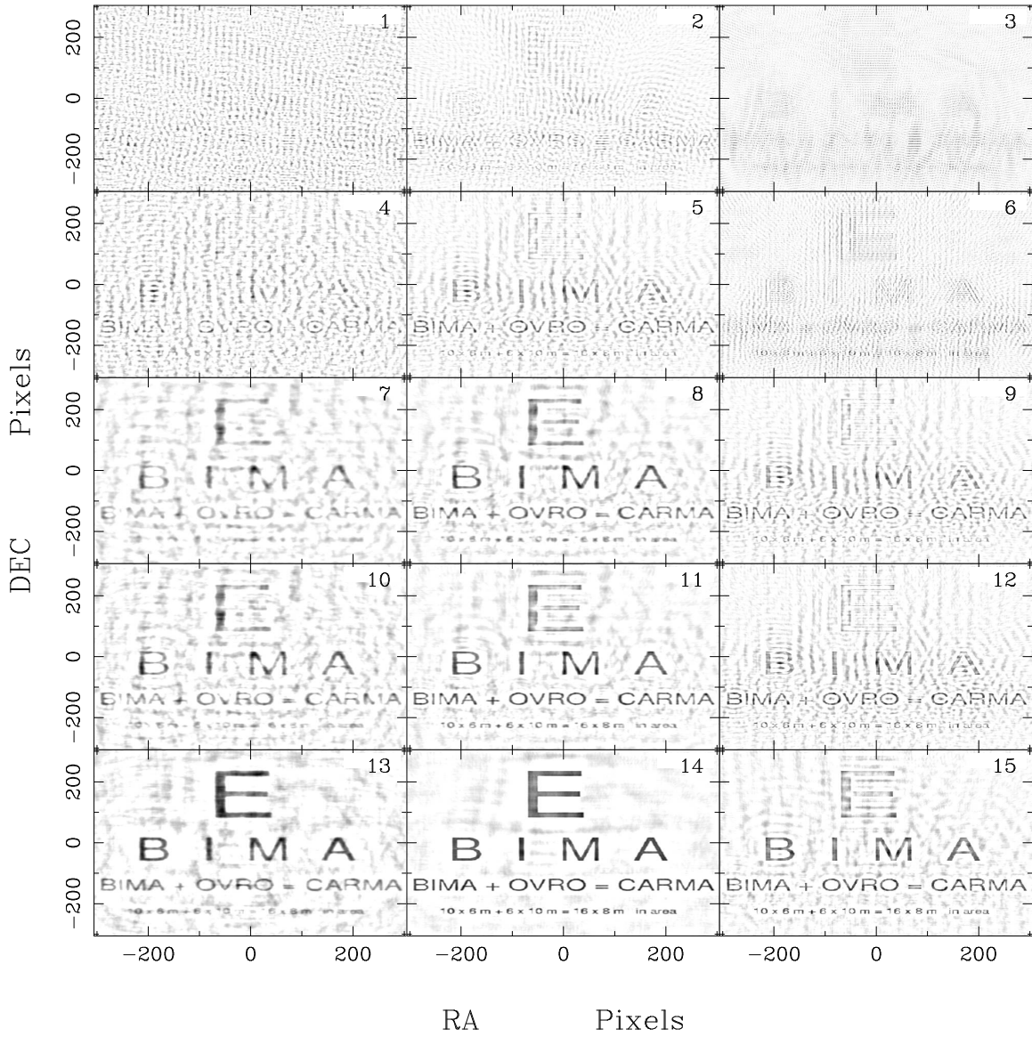
Fig. 6.— Eye chart imaged with different uv sampling: (row 1) six antennas, (row 2) ten antennas, (row 3) combined array without cross correlations between 10.4 m and 6.1 m antennas, (row 4) combined array with all cross correlations, (row 5) 27-antenna VLA scaled to the same resolution. (col 1) A single frequency, (col 2) MFS synthesis with 8% bandwidth, (col 3) MFS synthesis with array size scaled \times 2.5 .
