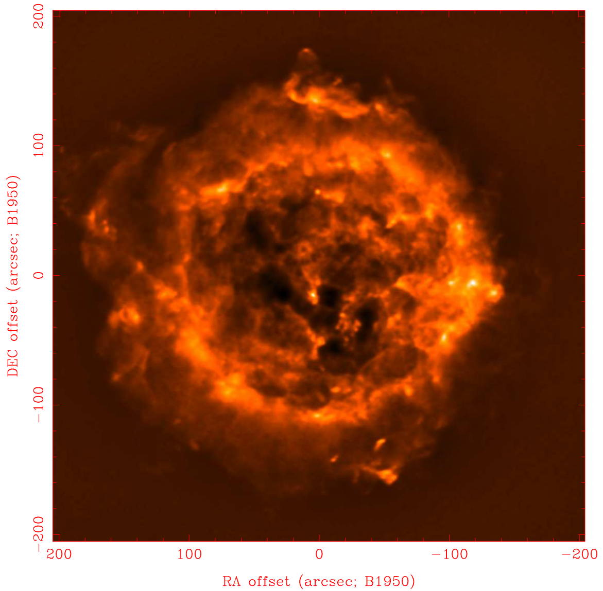
Fig. 3.— Model image of Cas A using observations at 4 configurations of CARMA and 2 frequency channels, 100 and 108 GHz. The resolution is 2.1'' \times 1.8''
